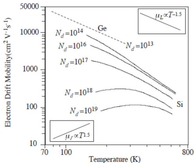
Fig. Q7b. The plot for drift mobility versus temperature for n -type Ge and n -type Si samples. Various donor concentrations for Si are shown, N_d are in \text{cm}^{-3} .
