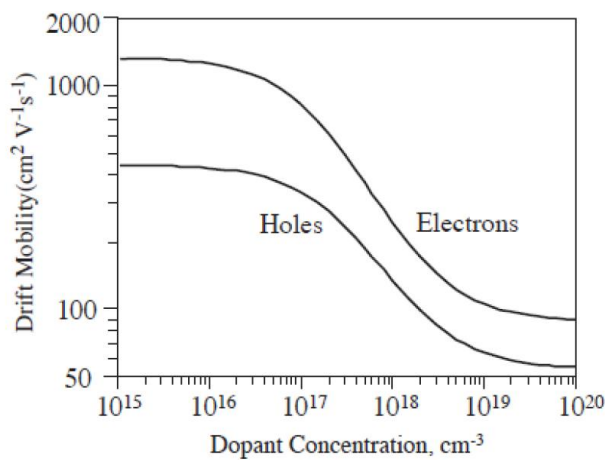
Fig. Q7a. The variation of the drift mobility with dopant concentration in Si for electron and holes at 300 K.
